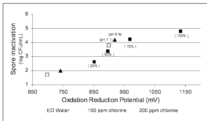
Figure 1—Relationship between oxidation-reduction potential (ORP) of 25%, 50%, 75%, and 100% EO water and chlorine with or without pH adjustment and log 10 reduction of Penicillium expansum spores treated for 60 s.
